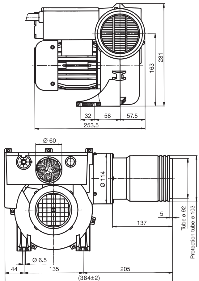
Installation dimensions in mm
